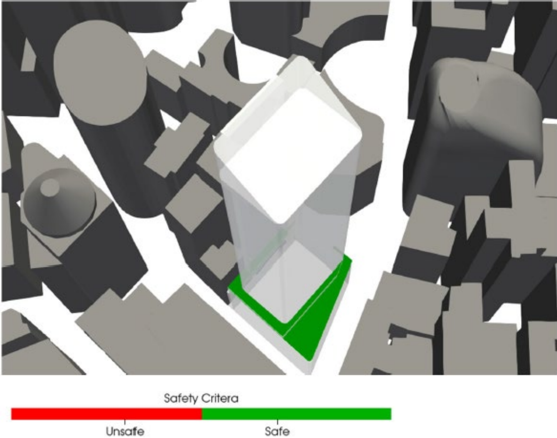
Figure 2-3 DCP Wind Safety Standard results
