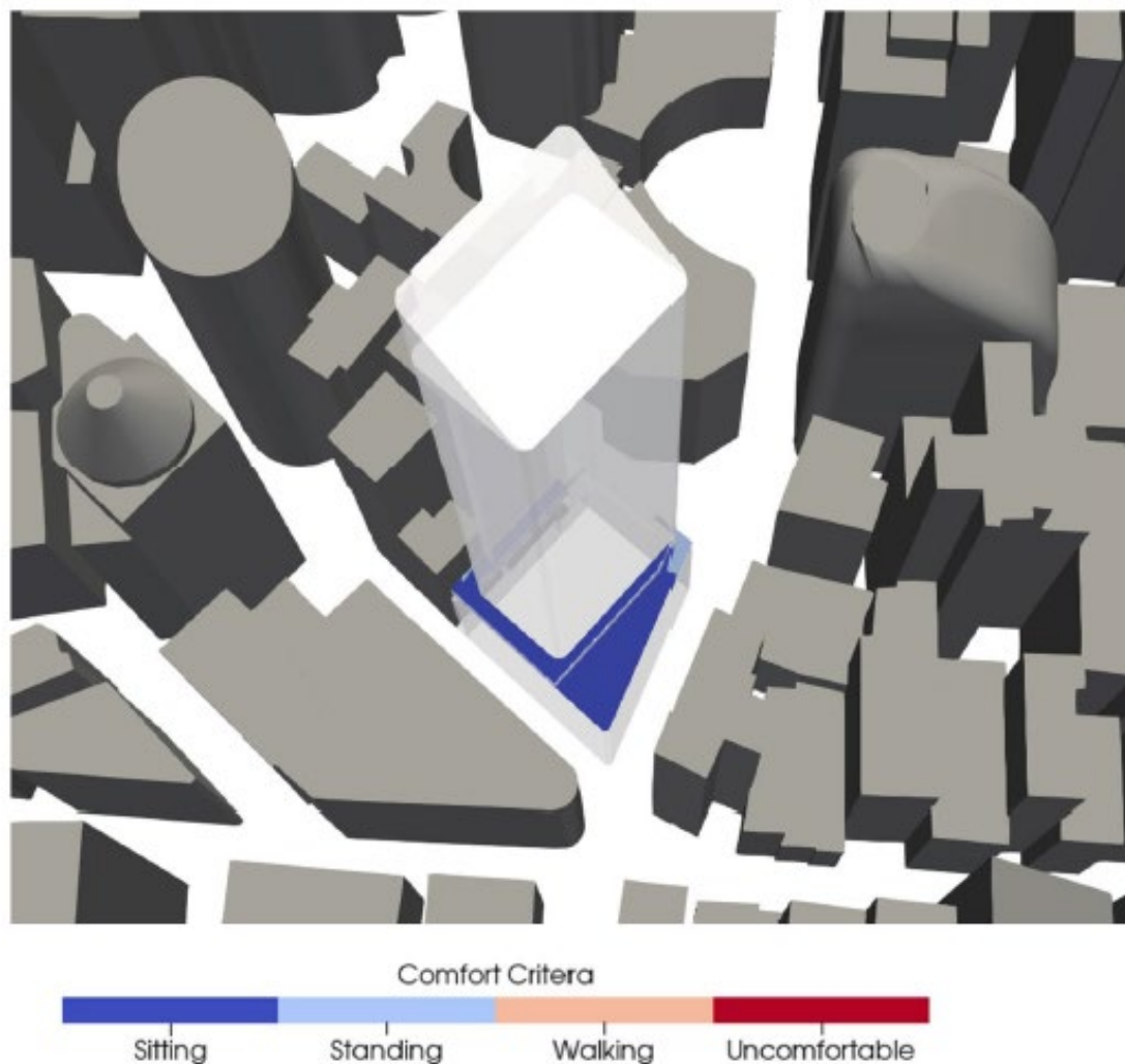
Figure 2-1 DCP Wind Comfort Standard results
