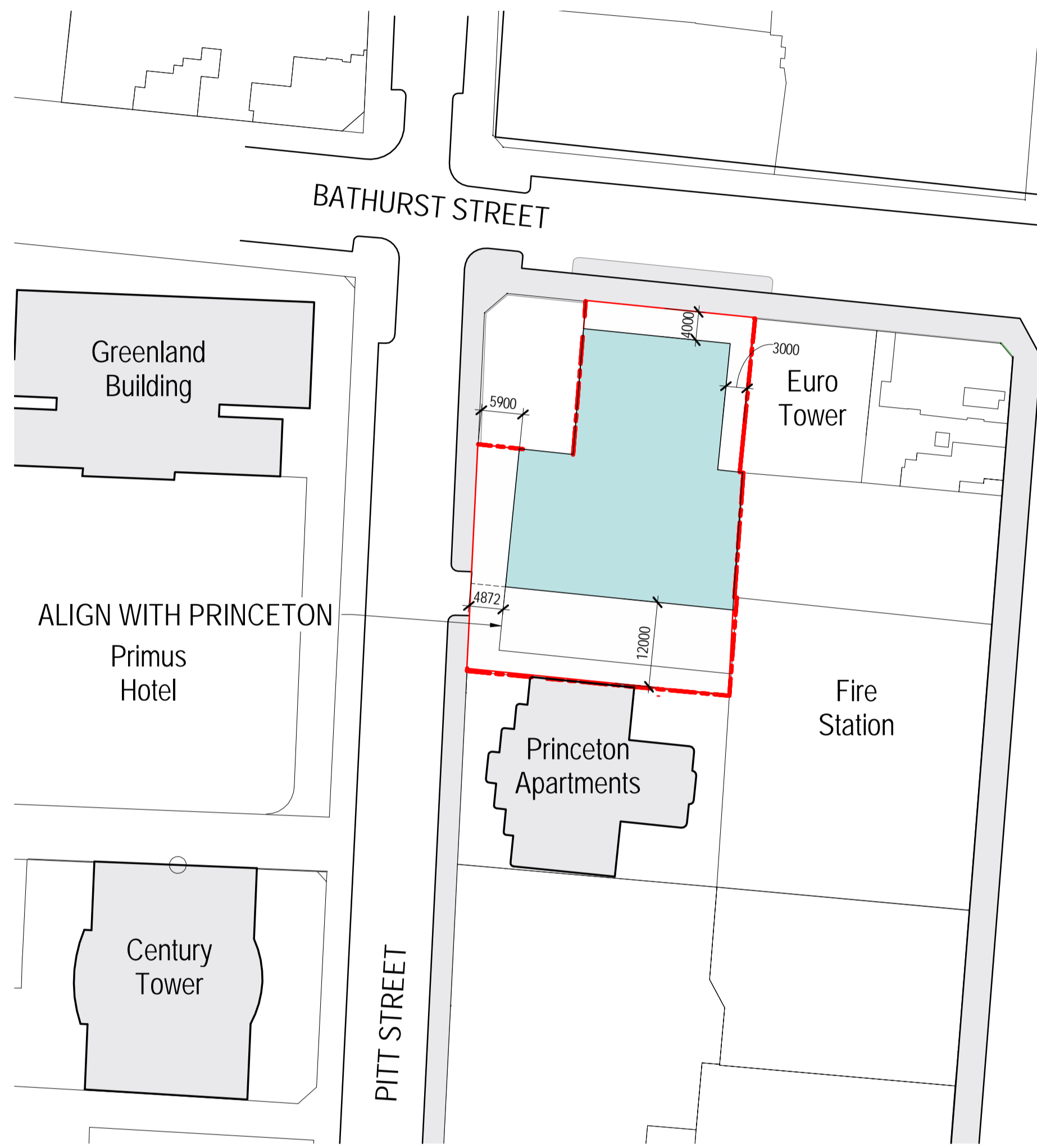
2 PROPOSED SETBACK RL 71.0 UPWARDS 1:600
