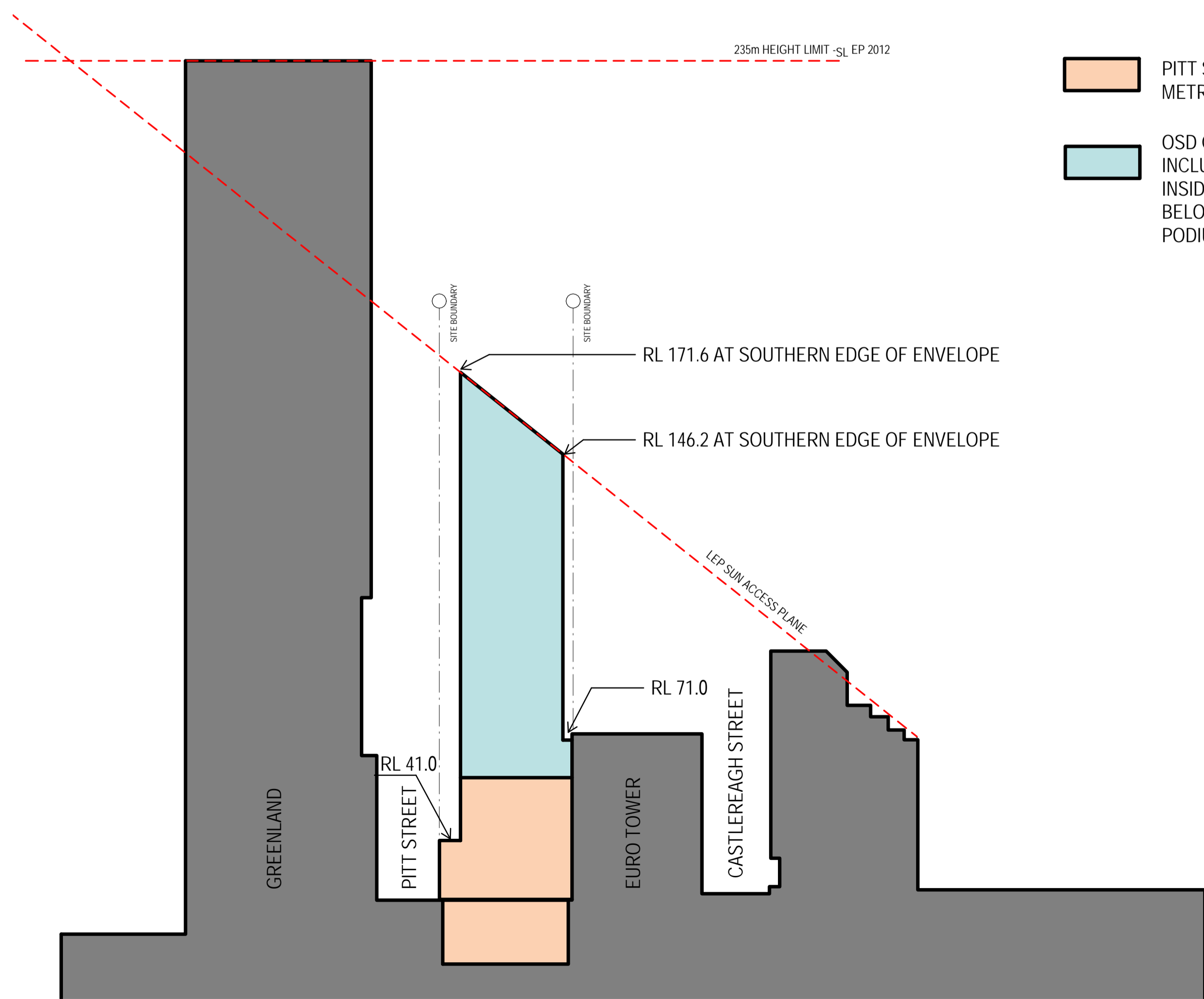
6 SECTION EAST WEST 1:1000
