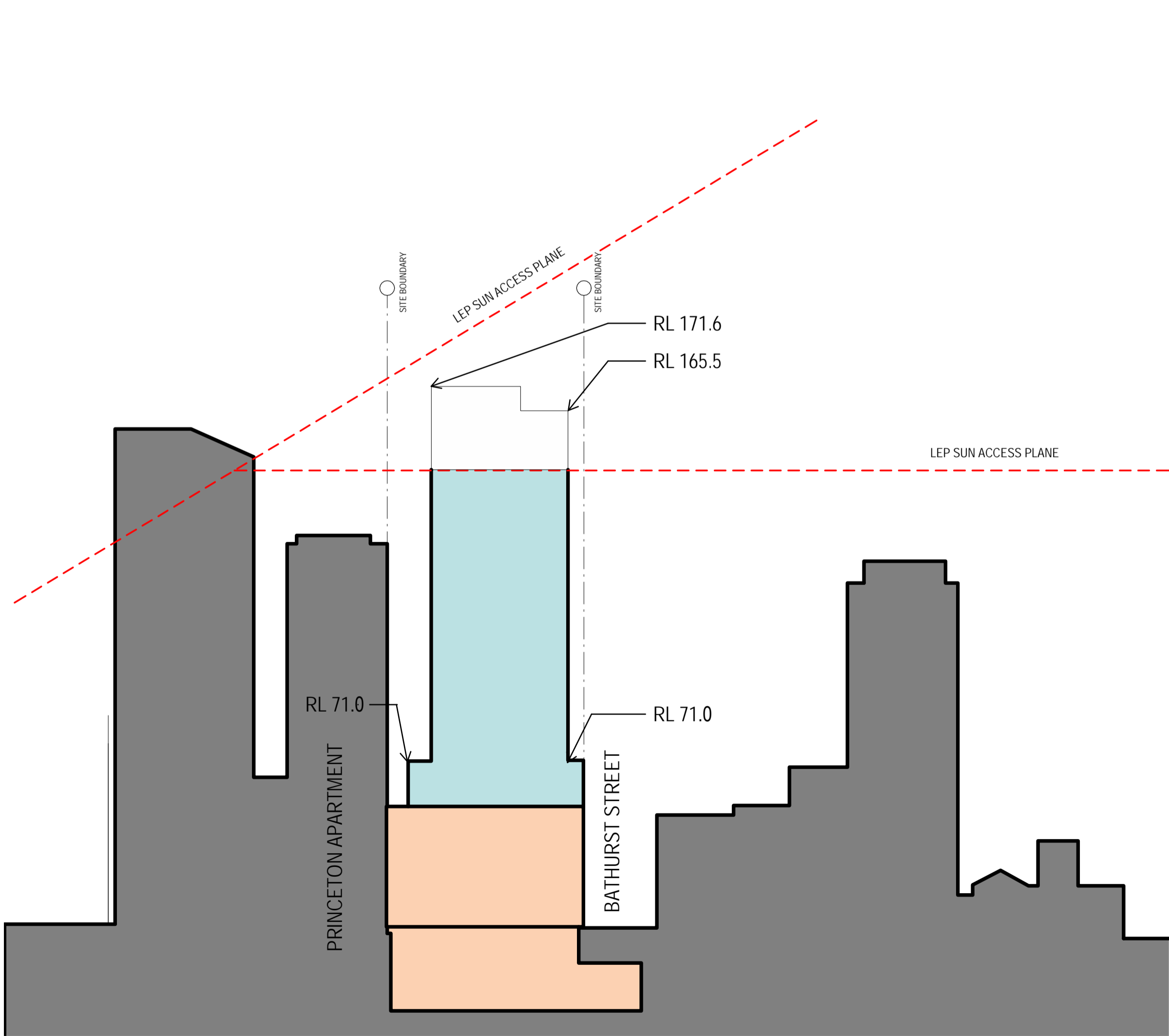
5 SECTION NORTH SOUTH 1:1000
